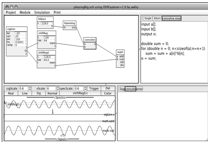
Figure 7—Similar display for phasing LSB generator.
