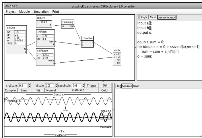
Figure 6—Components of a simple phasing USB generator.
