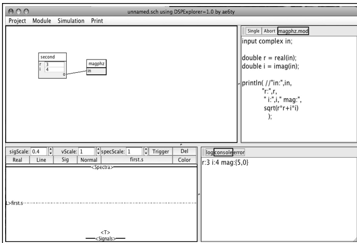
Figure 3—Using parameters to provide constants.
