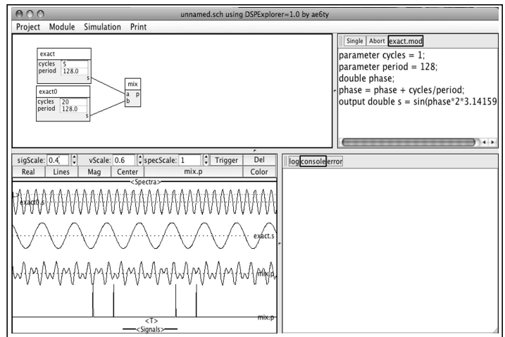
Figure 4—Generating and mixing two signals.
