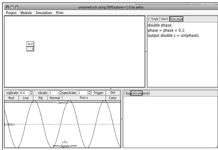
Figure 2—Default screen after correcting error.
