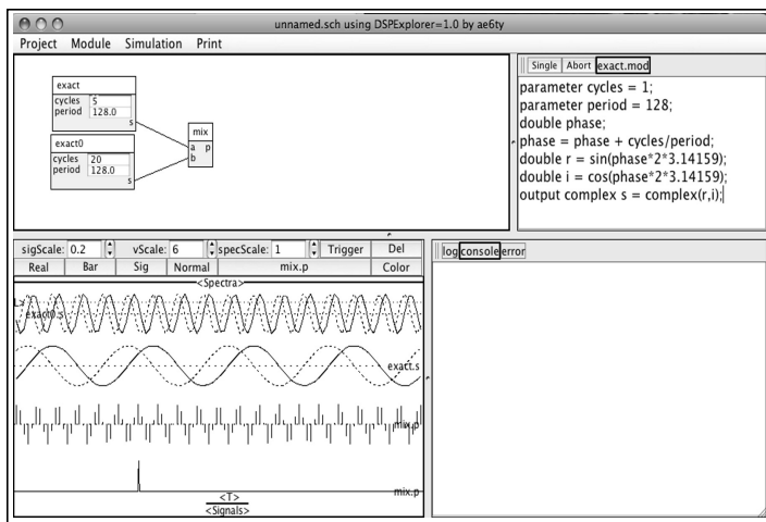
Figure 5—Mixing complex signals.
